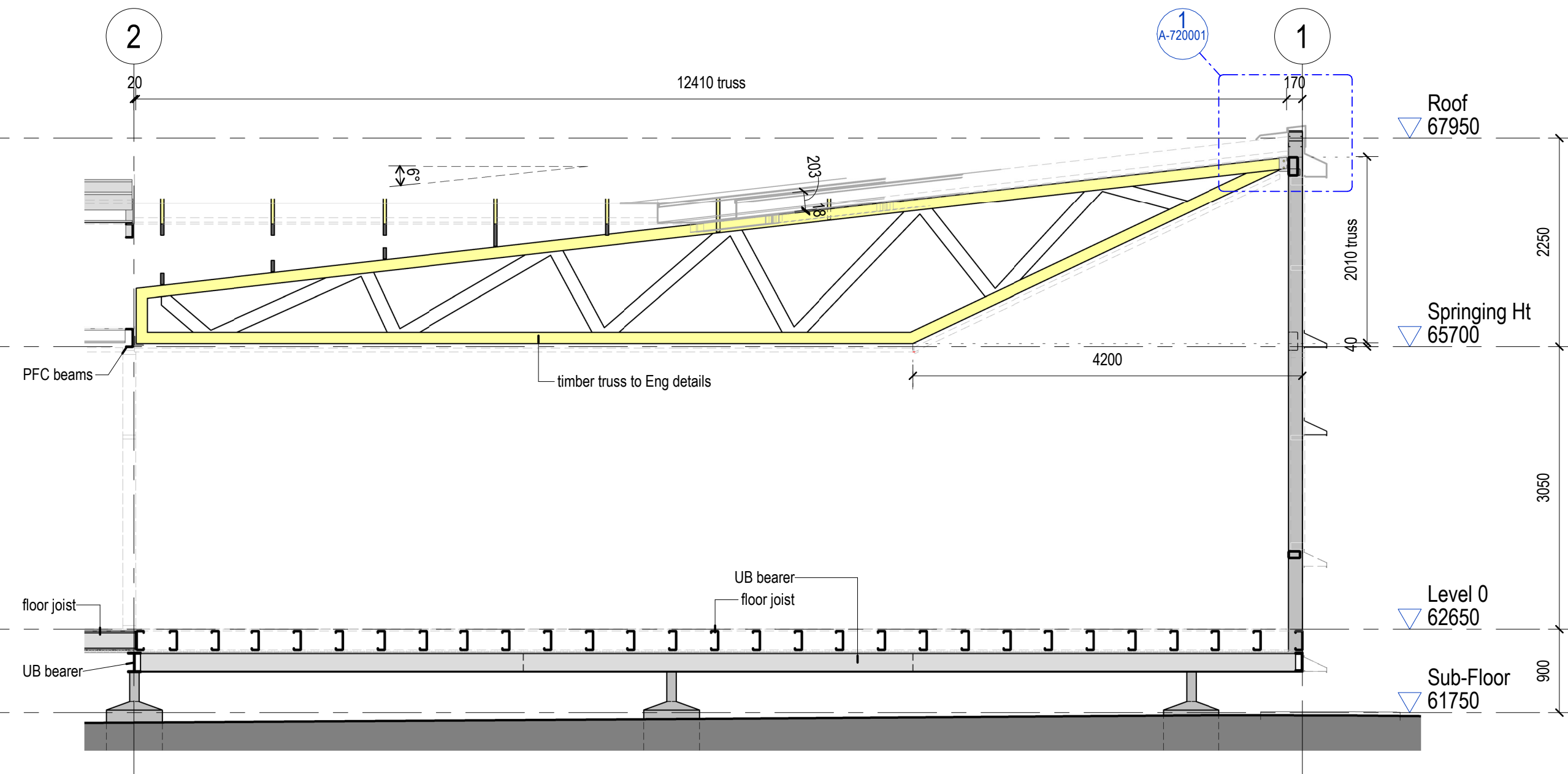
2 Detail Section - Raking Ceiling 1 : 50 Truncated Truss Configuration
