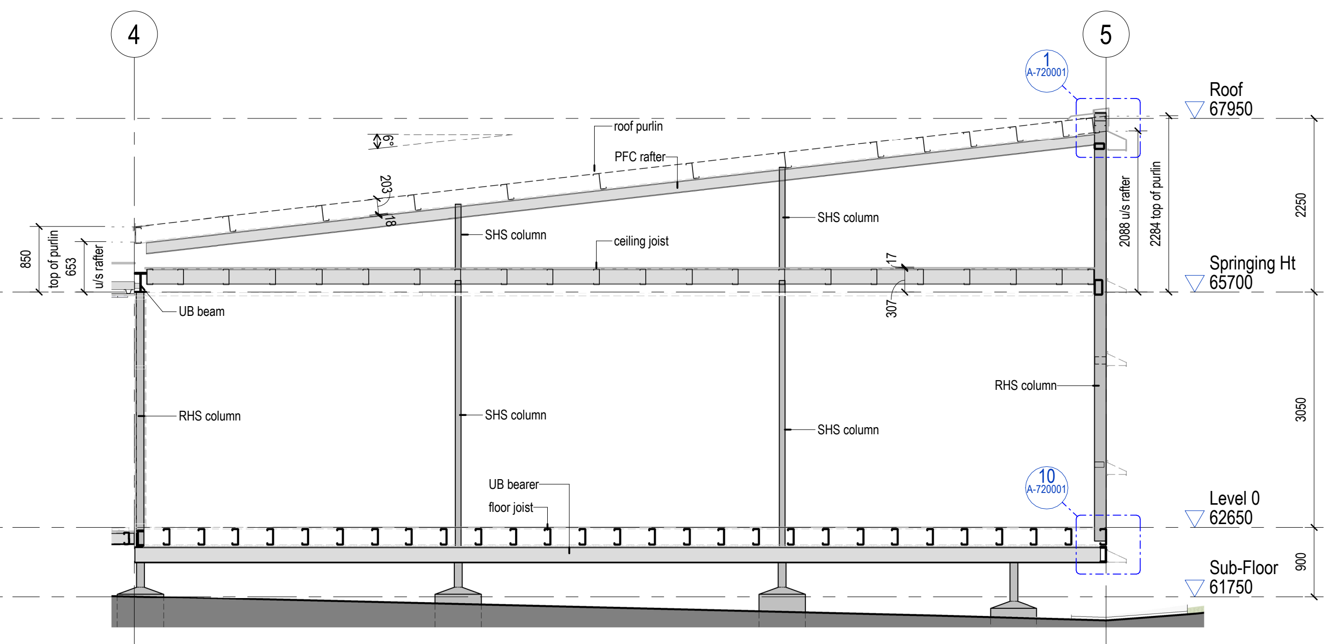
4 Detail Section - Plant Room Over Training 1 : 50 Steel Roof Purlins
