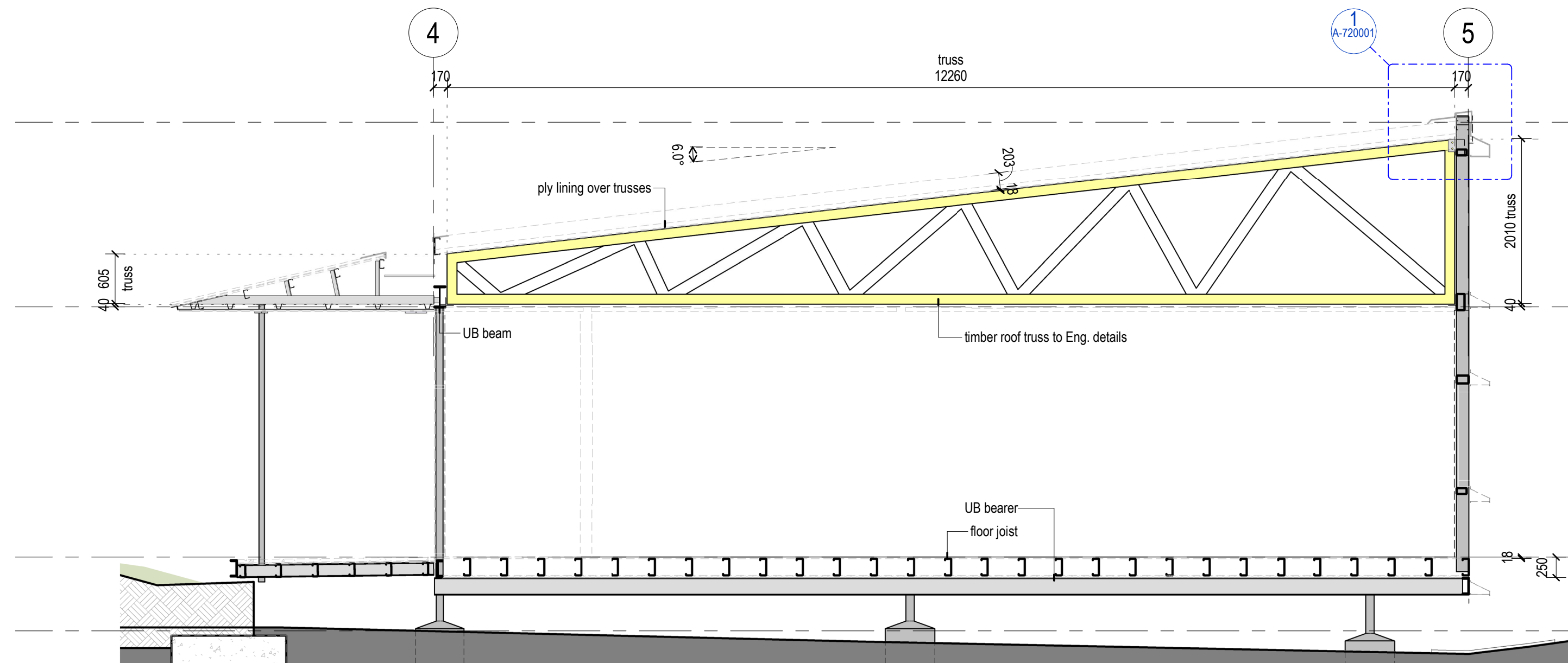
1 Detail Section - Typical 1 : 50 Full Truss Configuration
