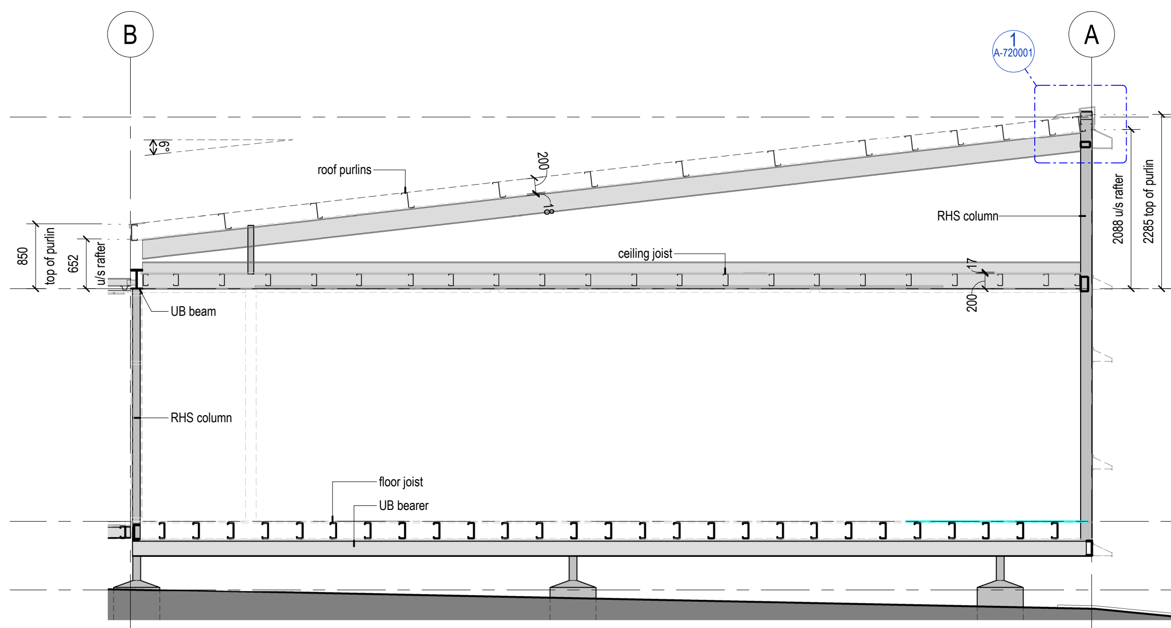
3 Detail Section - Plant Room Over Offices 1 : 50 Steel Roof Purlins
